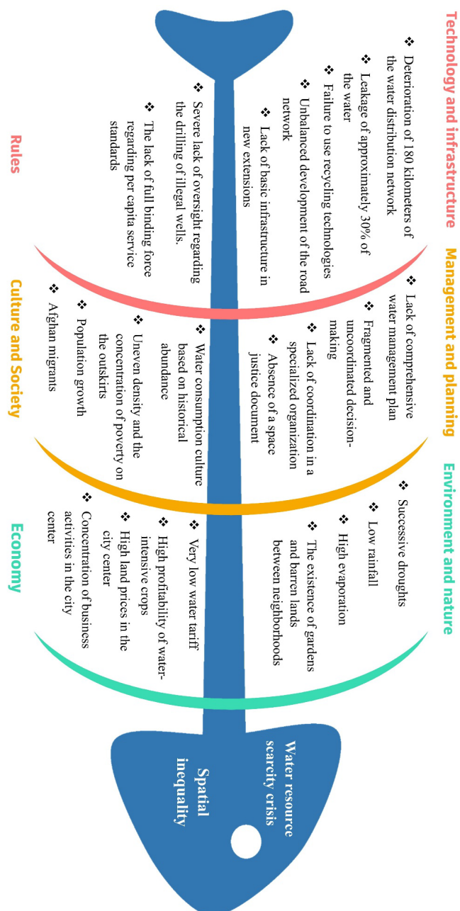
Figure 5. Fishbone diagram analysis
